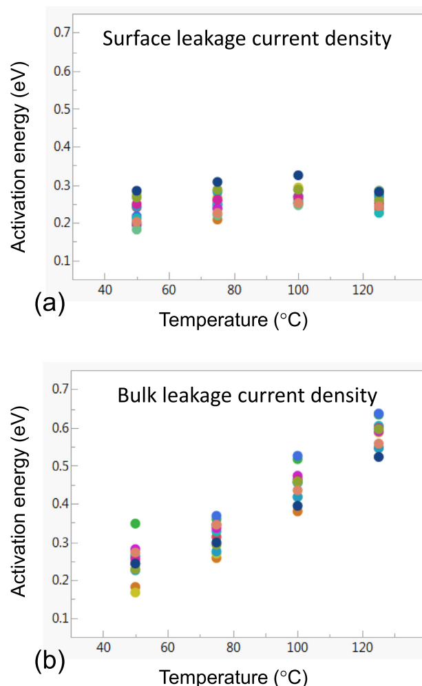
FIG. 13. Wafer-scale activation energy data of (a) the surface leakage current density and (b) the bulk leakage current density as a function of measurement temperature.
