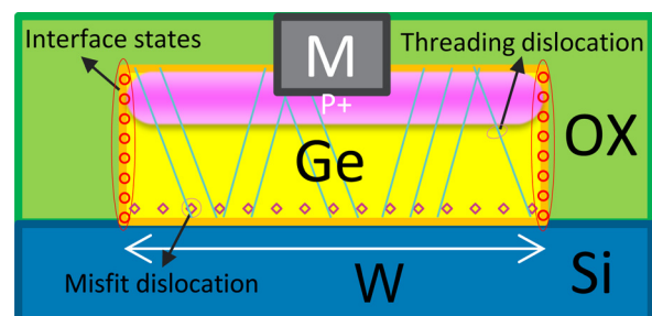
FIG. 6. Schematic diagram illustrating the dark current modeling of VPIN GePDs.
