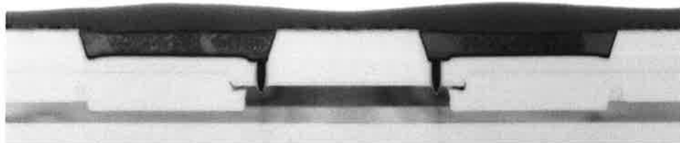
Figure 3: Cross section picture of a horizontal Ge diode, after Cu metallization.
