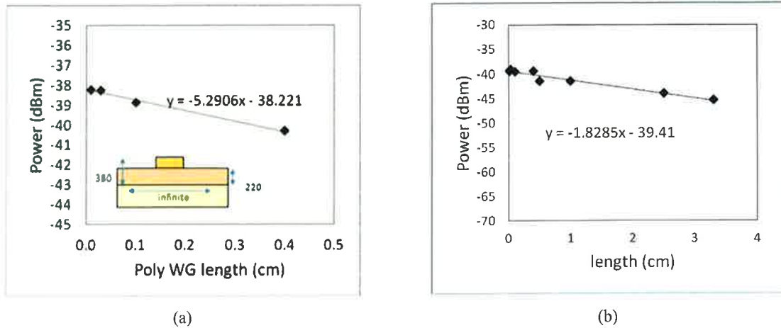
Figure 4: Transmitted power as a function of WG length for (a) 350nm wide hybrid poly Si/Si WG showing 5.3dB/cm loss, and (b) 400nm wide Si WG, with an average of 1.85dB/cm loss.
