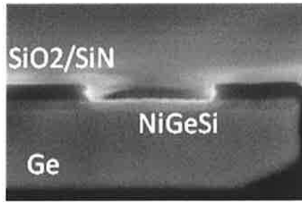
Figure 2: XSEM image of a local silico-germanide.
