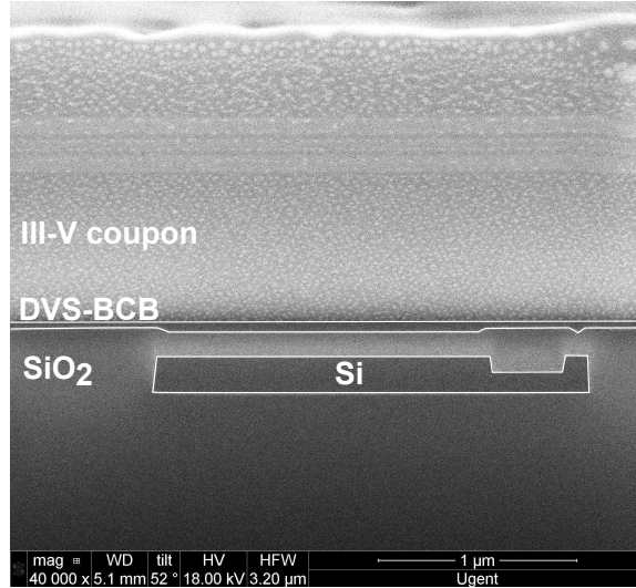
Figure 2: Cross section of a coupon transfer printed on BCB-coated planar SOI
