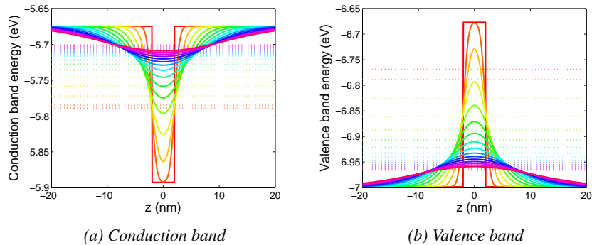
Figure 2.5: Simulation for many different diffusion lengths, varying from 0 nm to 15 nm (steps of 1 nm).
