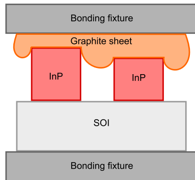
(a) Illustration of multiple die bonding with graphite sheet to spread the pressure.
