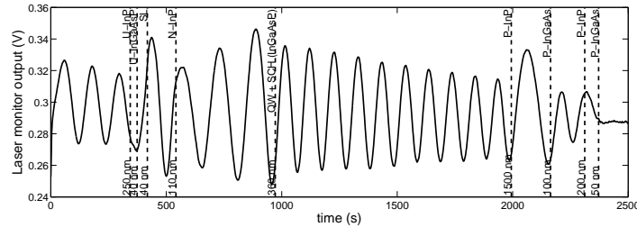
Figure 3.12: RIE etch test on a dummy sample. As can be seen, the period change between the SCH and p-InP is only fully clear when one sees at least a complete period. Note that in the normal process, one starts etching from the other side.
