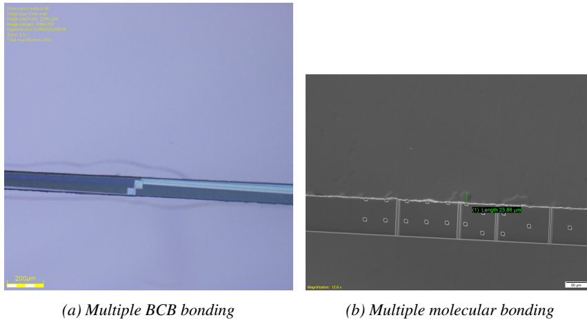
(a) Multiple BCB bonding (b) Multiple molecular bonding Figure 2.17: Minimizing the gap region for both bonding techniques to 100 μm. The top and bottom of the picture show the two bonded InP dies. In the middle the exposed waveguide structures are visible.
