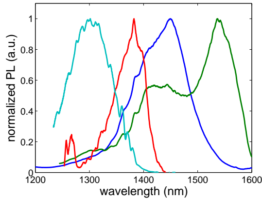
Figure 2.12: The photoluminescence spectra from the four generated band gaps transposed on one graph
