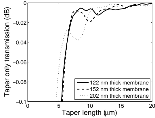
Figure 4.13: Transmission through the taper as a function of the taper length. The III-V tip was 700 nm wide for all membranes.
