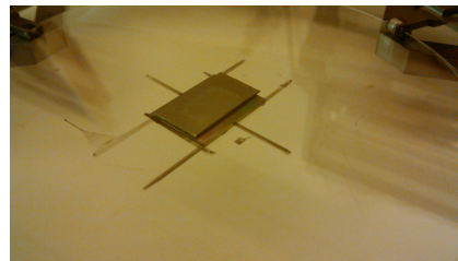
(b) Sample ready to load for bonding. Two InP dies are positioned on a SOI sample, with graphite sheet covering them. Everything is sandwiched between two glass wafers.
