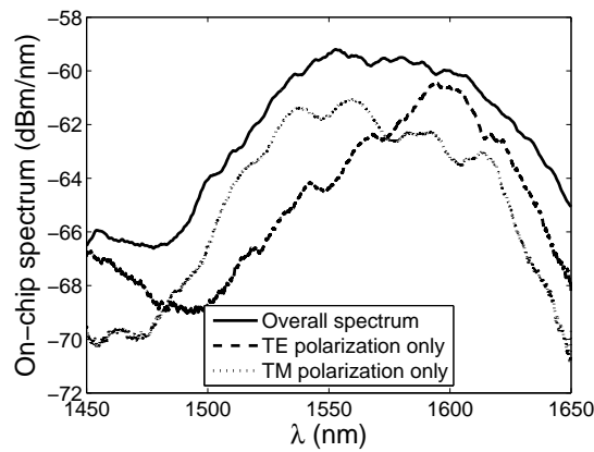
(b) Co-propagating spectrum of a 37 \mu\text{m} long LED.
