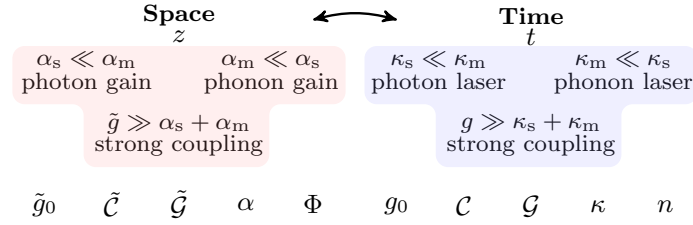
Figure 3.2: Symmetry of circuit and cavity optomechanics. Each temporal optomechanical effect has a spatial symmetry partner. Thus, the description of these effects can be cast in terms of conceptually similar figures of merit. The scheme assumes a red-detuned optical probe; “gain” and “laser” should respectively be replaced by “loss” and “cooling” for a blue-detuned optical probe. The meaning of the figures of merit is discussed in the main text.
